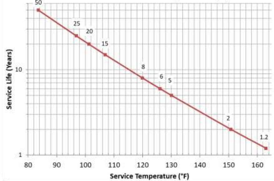
DTN2070 Service Life vs. Temperature (°F)
